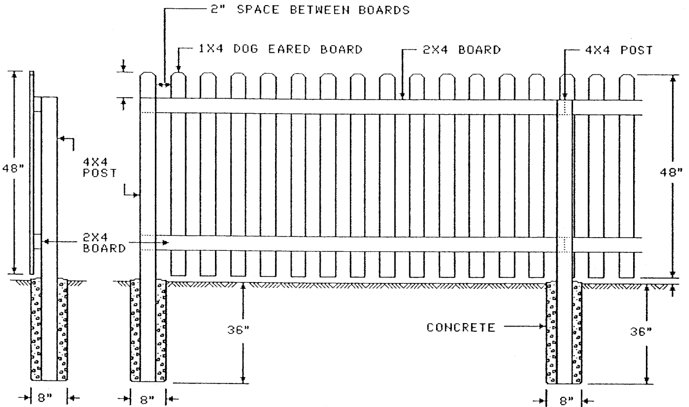
(SIDE VIEW)
