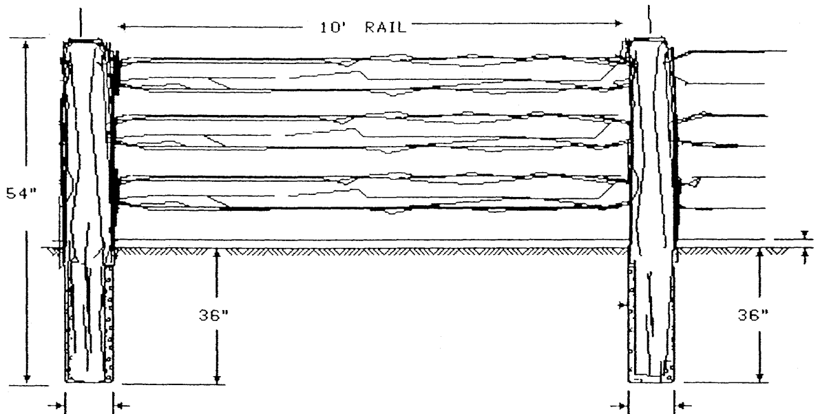
(ELEVATION VIEW)
