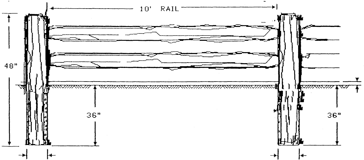
(ELEVATION VIEW)
